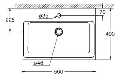
39 474 00H Lavabo suspendu 50 cm
