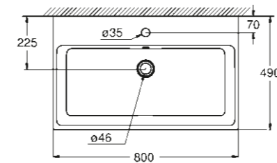
39 469 00H Lavabo suspendu 80 cm
