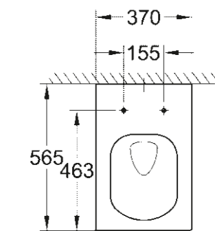
39 244 00H WC suspendu Triple Vortex
