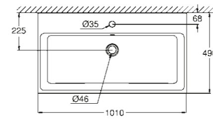
39 386 00H Lavabo suspendu 100 cm
